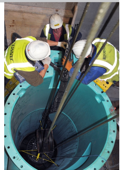
Installation process using BPL's latch lift system
